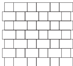
Flemish Bond
